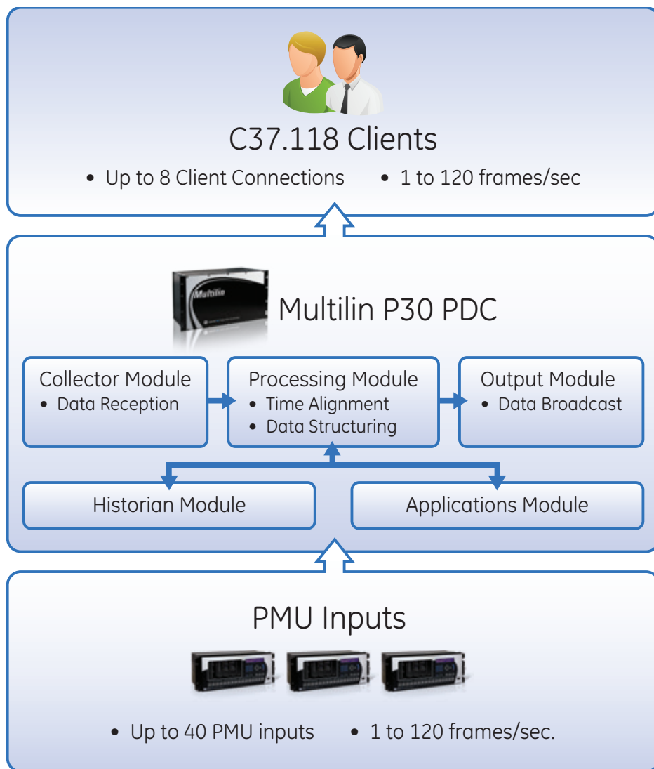
Multilin P30 Phasor Data Concentrator product architecture
