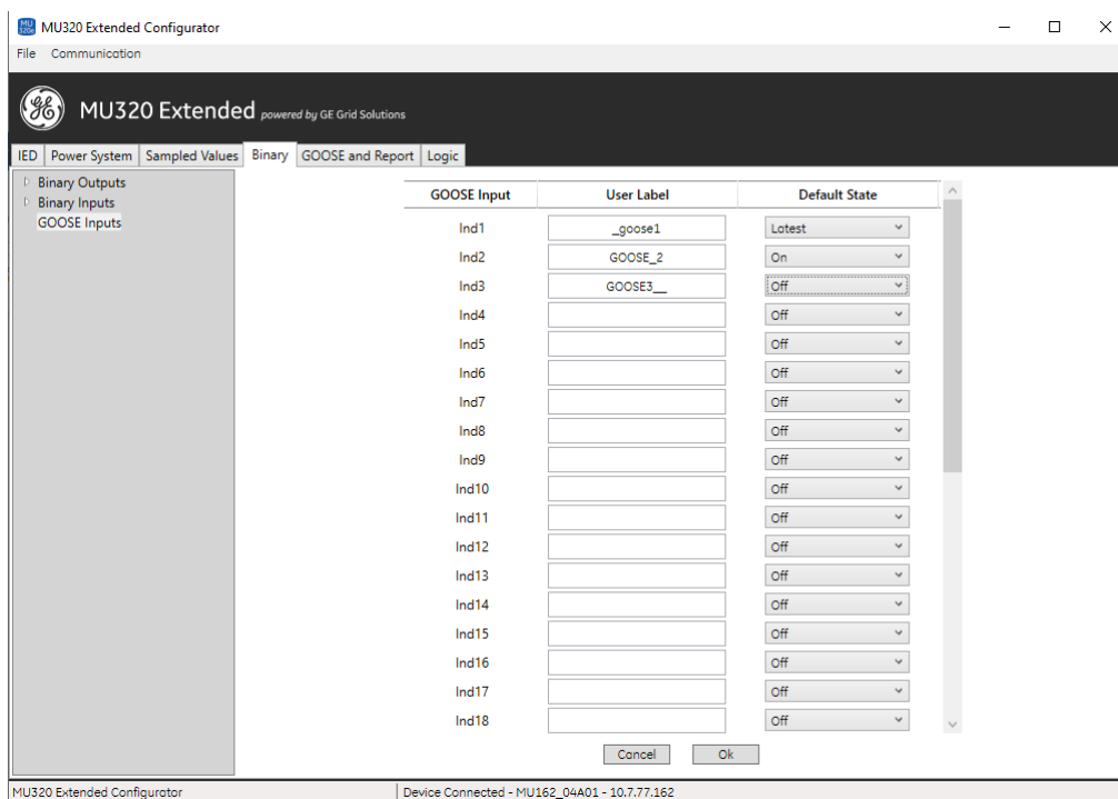
GOOSE Inputs Configuration
