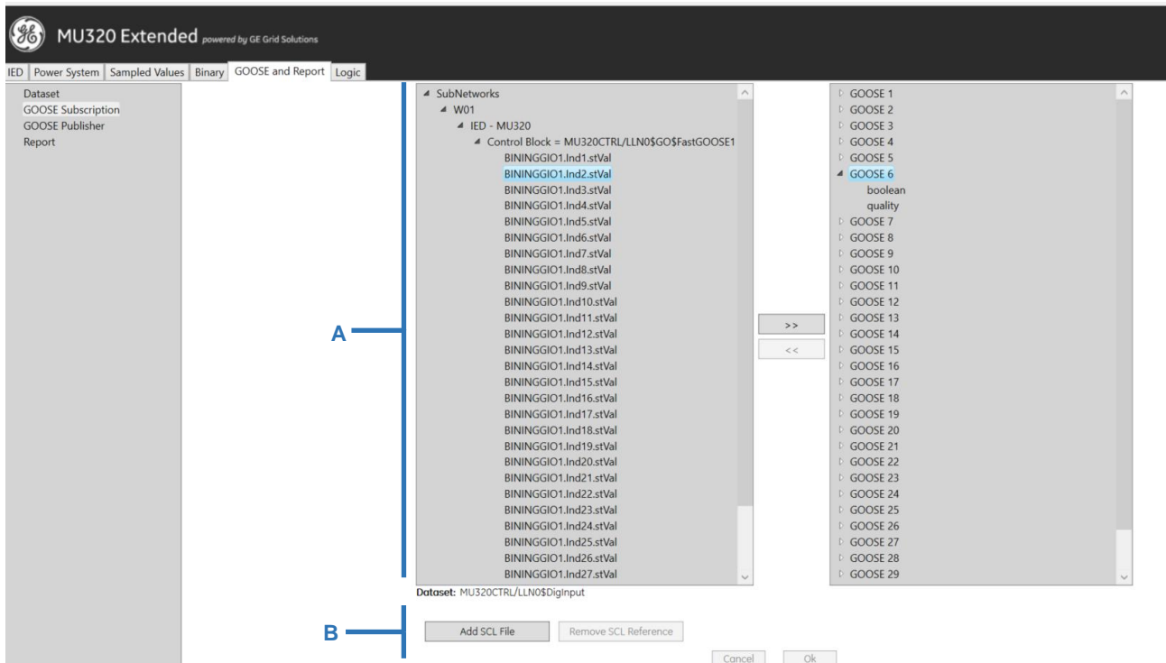
GOOSE Subscription Configuration Screen
