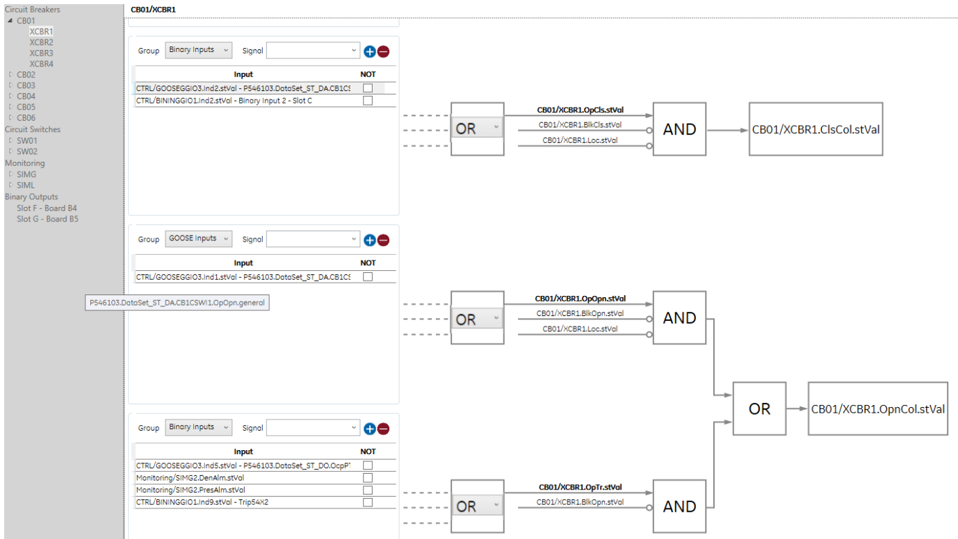
Binary Inputs to Data Model for logics with more than one element
