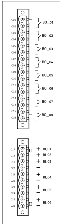
Binary board model B4
