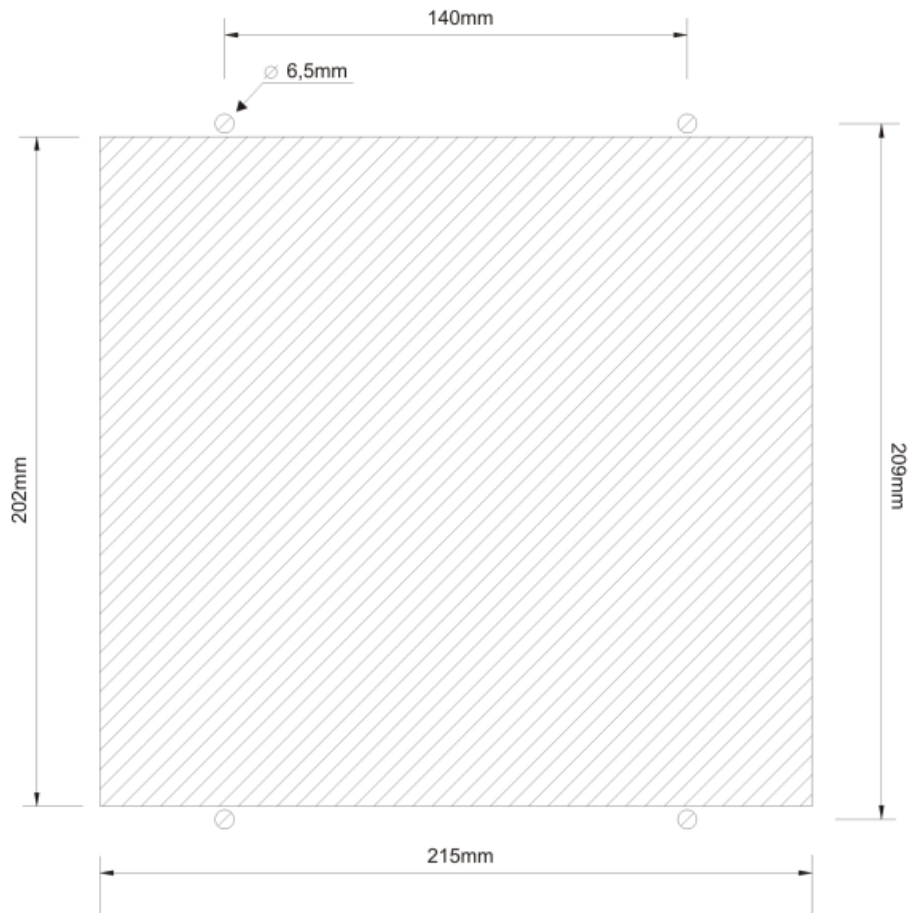
Panel cutout for MU320E installation
