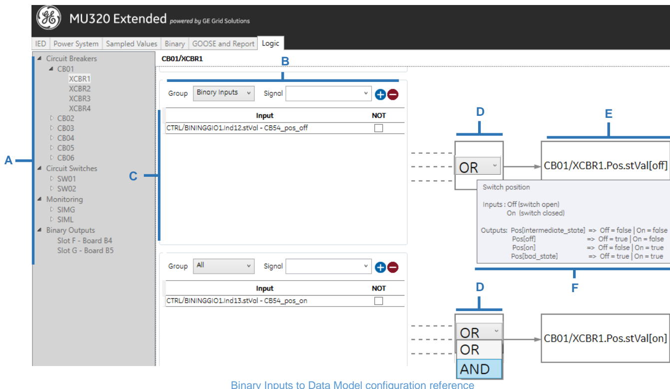
Binary Inputs to Data Model configuration reference
