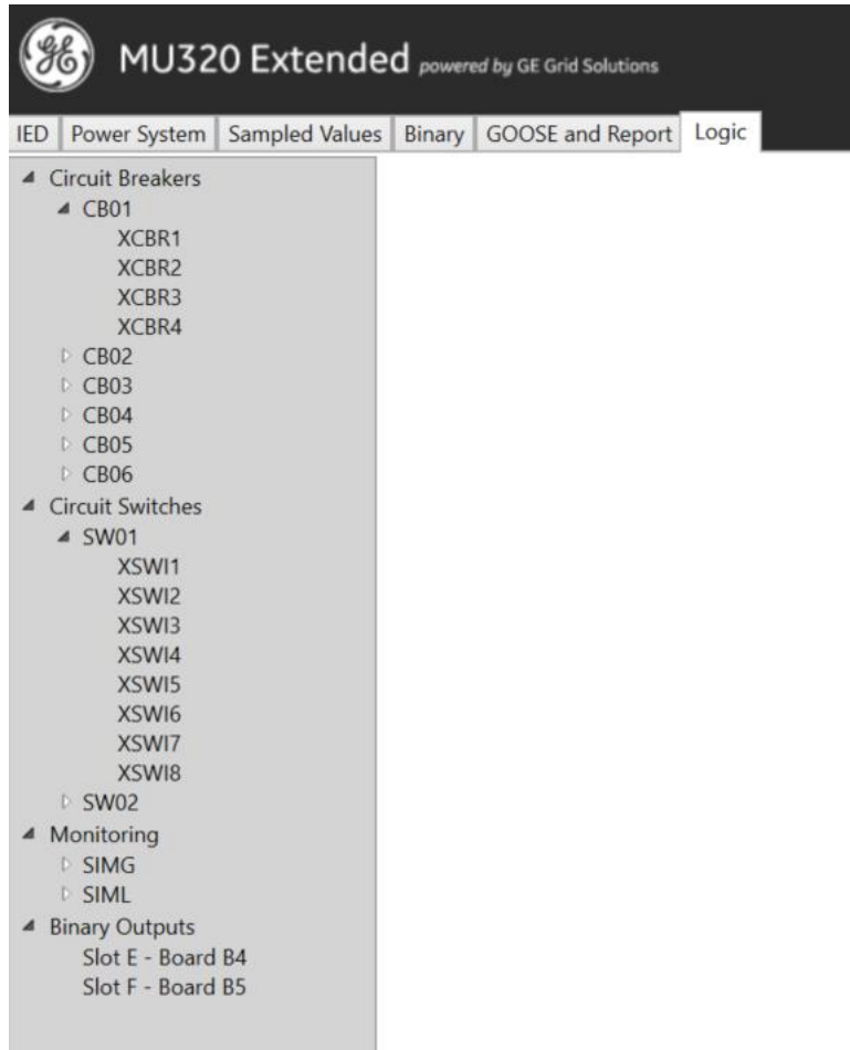
Logic Configuration Main Screen
