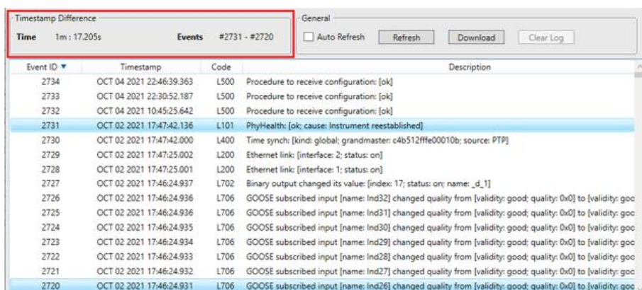
Example for analysis of Log events
