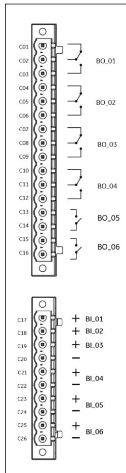
Binary board model B5
