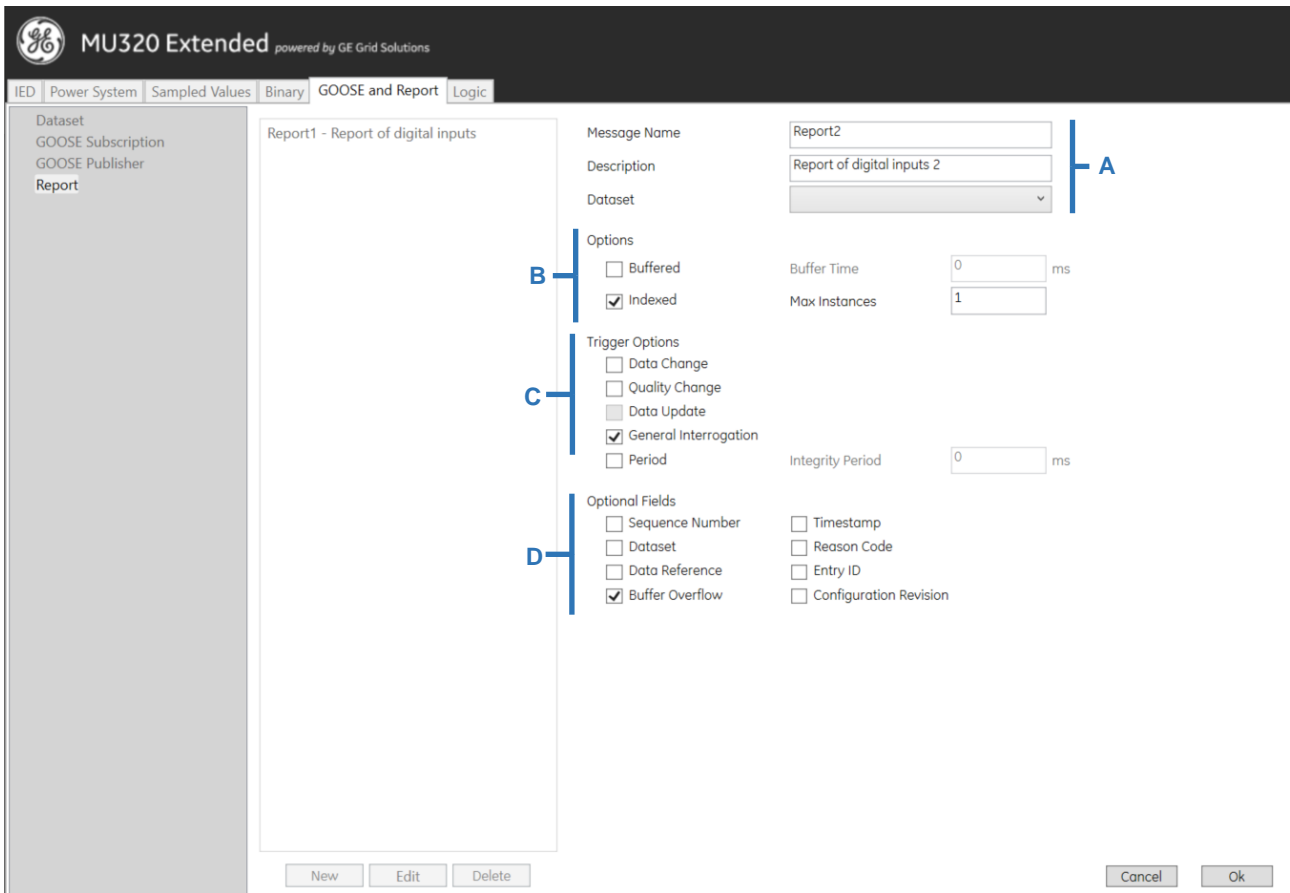
GOOSE Publisher Configuration Screen
