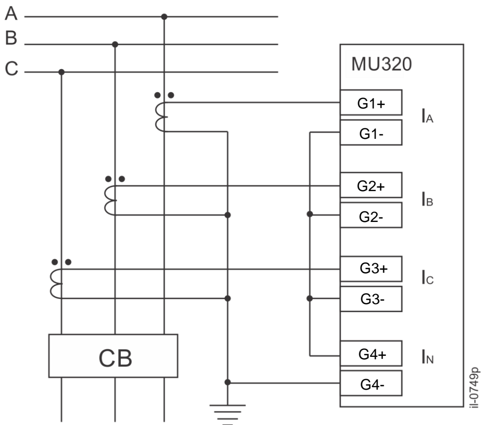
Typical current connection diagram
