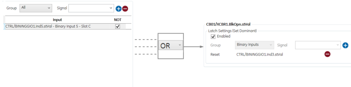
Circuit Breaker Opening Block by latching logic
