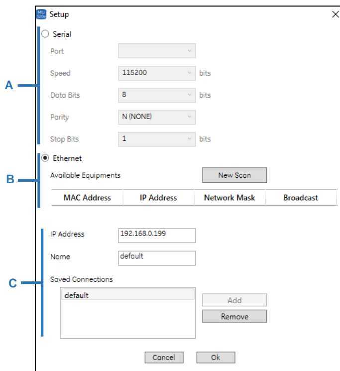
Communication Screen
