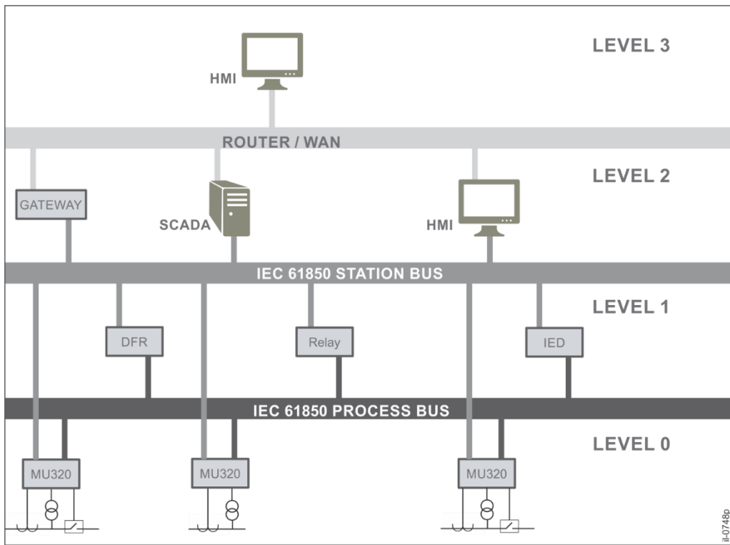
Application example using the MU320E
