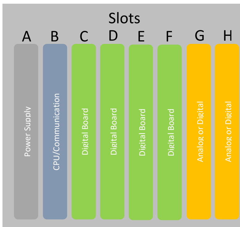
MU320E slots composition
