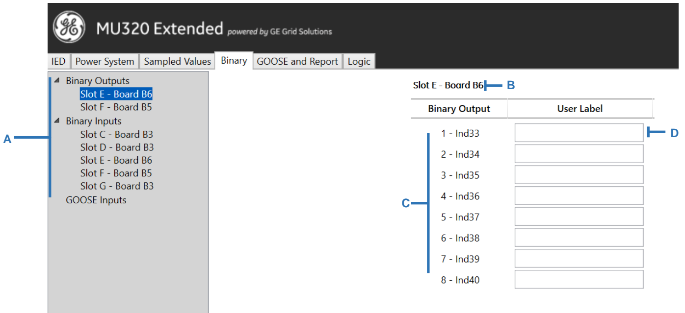
User Label configuration
