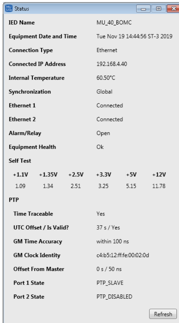
Status Screen
